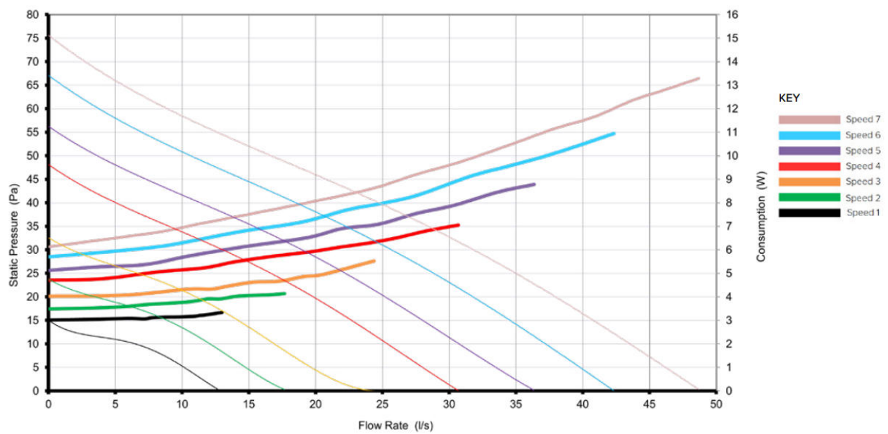
Normal Speed performances' curves V 1 to V 7 (Static pressure/FlowRate/Consumption)
